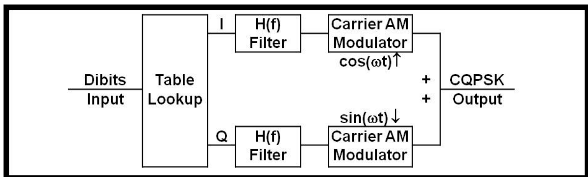
Figure 37– CQPSK Modulator
