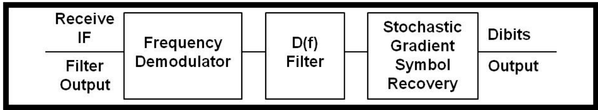
Figure 38– QPSK Demodulator
