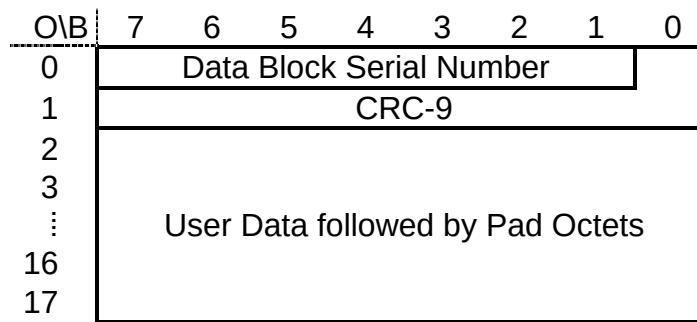
Figure 19 – Confirmed Data Packet Data Block
