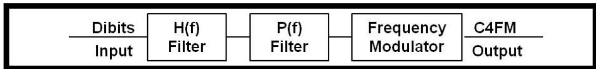
Figure 36– C4FM Modulator
