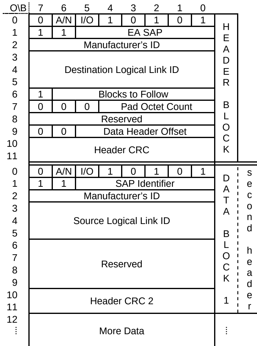
Figure 25 – Unconfirmed Enhanced Addressing Packet Header Format
